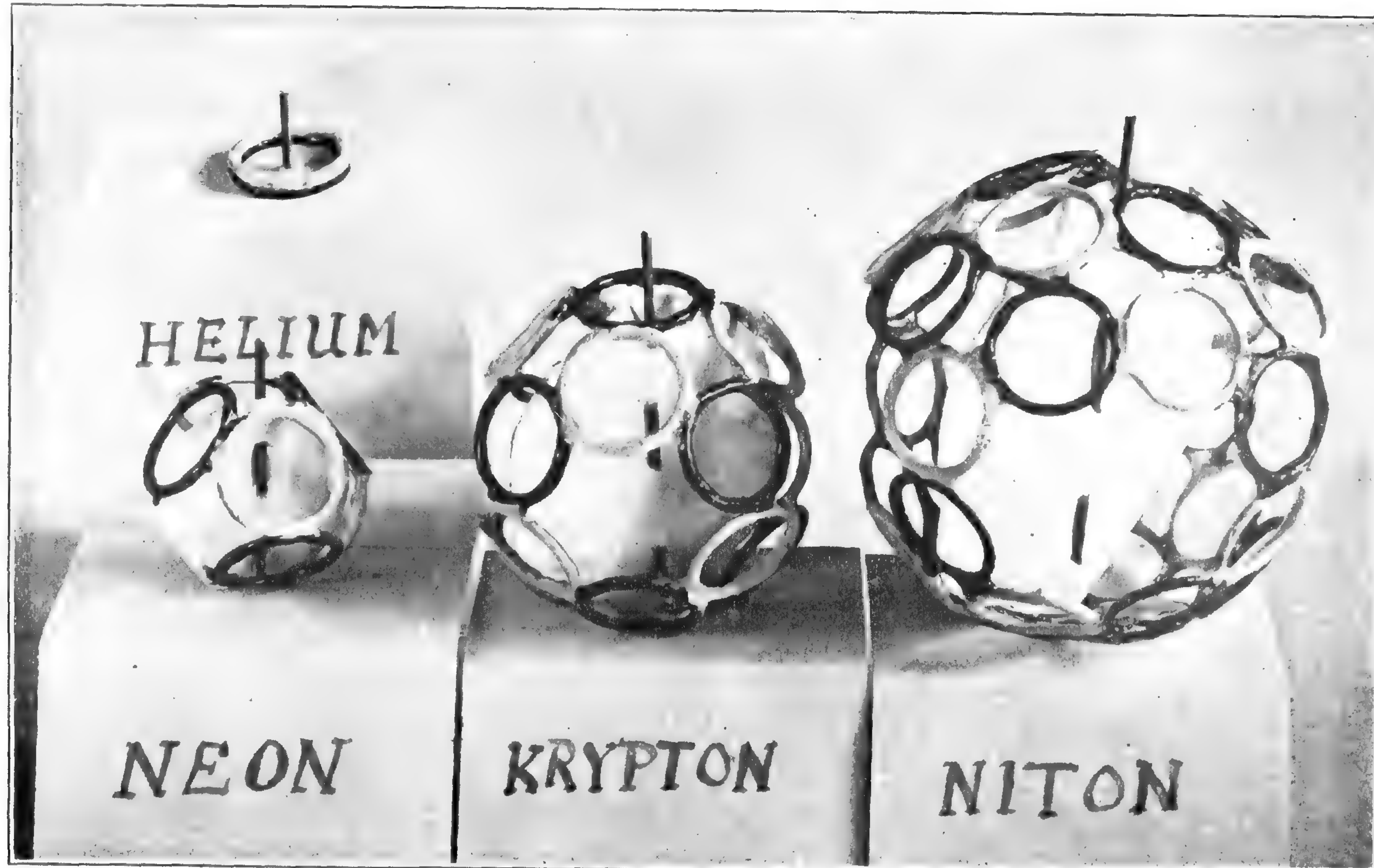
PLATE 1. MODELS OF THE ELECTRON SHELLS.
